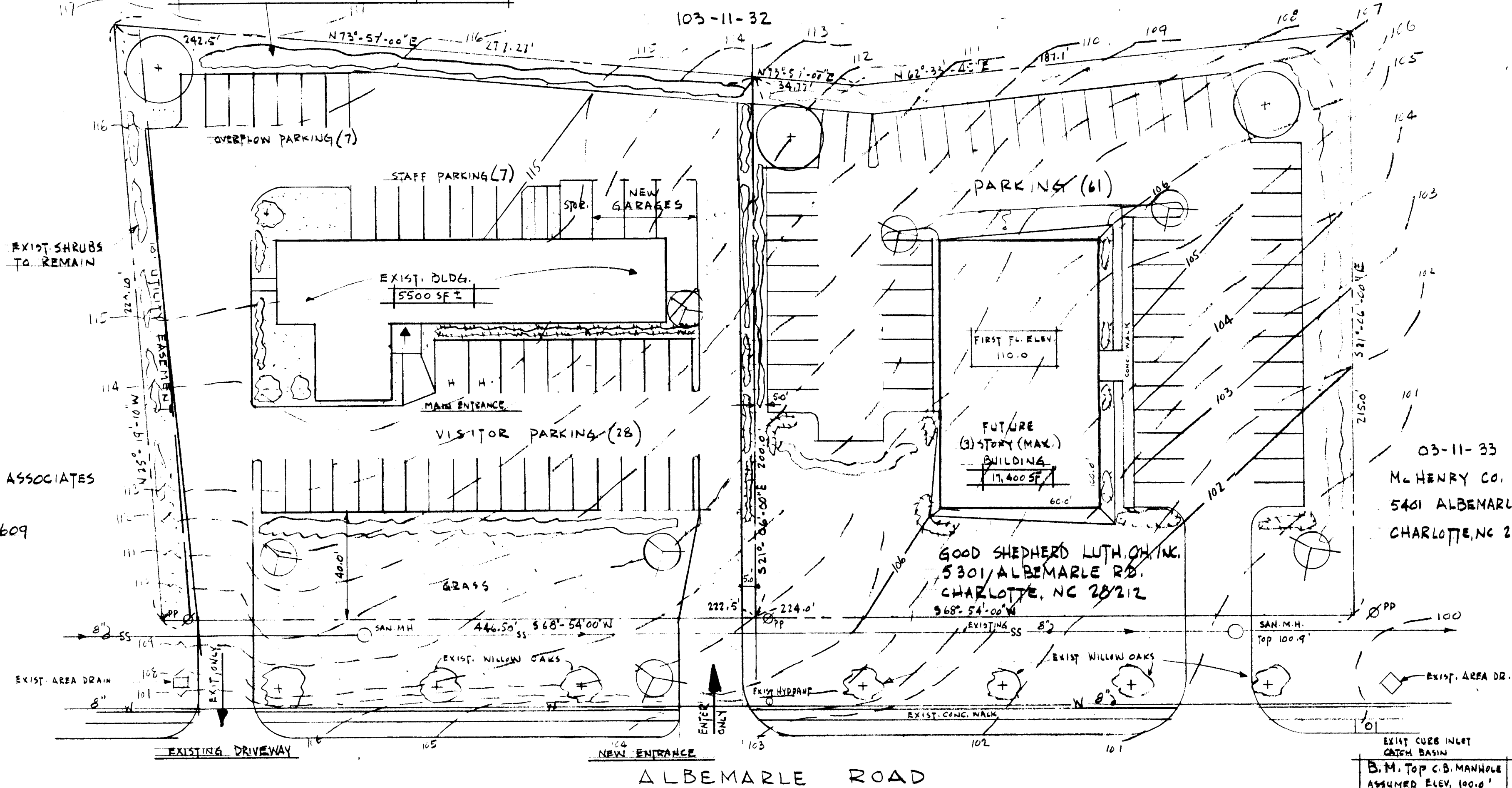
SITE DEVELOPMENT PLAN SCALE: 1"=30'
