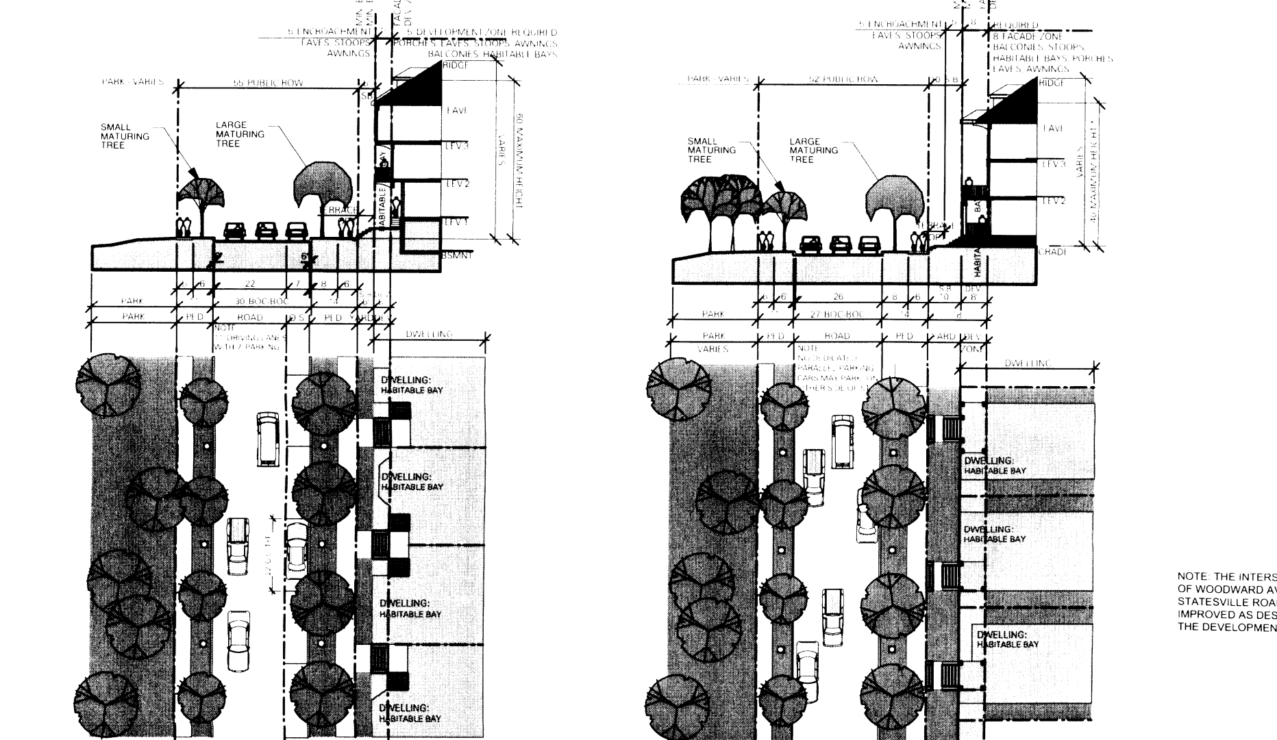
2MF Park Edge - Residential Street Multi Family - Park Edge - NS 55 Anita Stroud & Park Extension Street Section - 5 S.B. Two-Lane Two-Way Residential Street w/ Dedicated On-Street Parking (O Side) 2SF Park Edge - Medium Residential Street Single Family - Attached/Detached - UR2 52 Park Edge Road Street Section - 5 S.B. Two-Lane Two-Way Residential Street with Parallel Parking (non-striped) - Either Side
