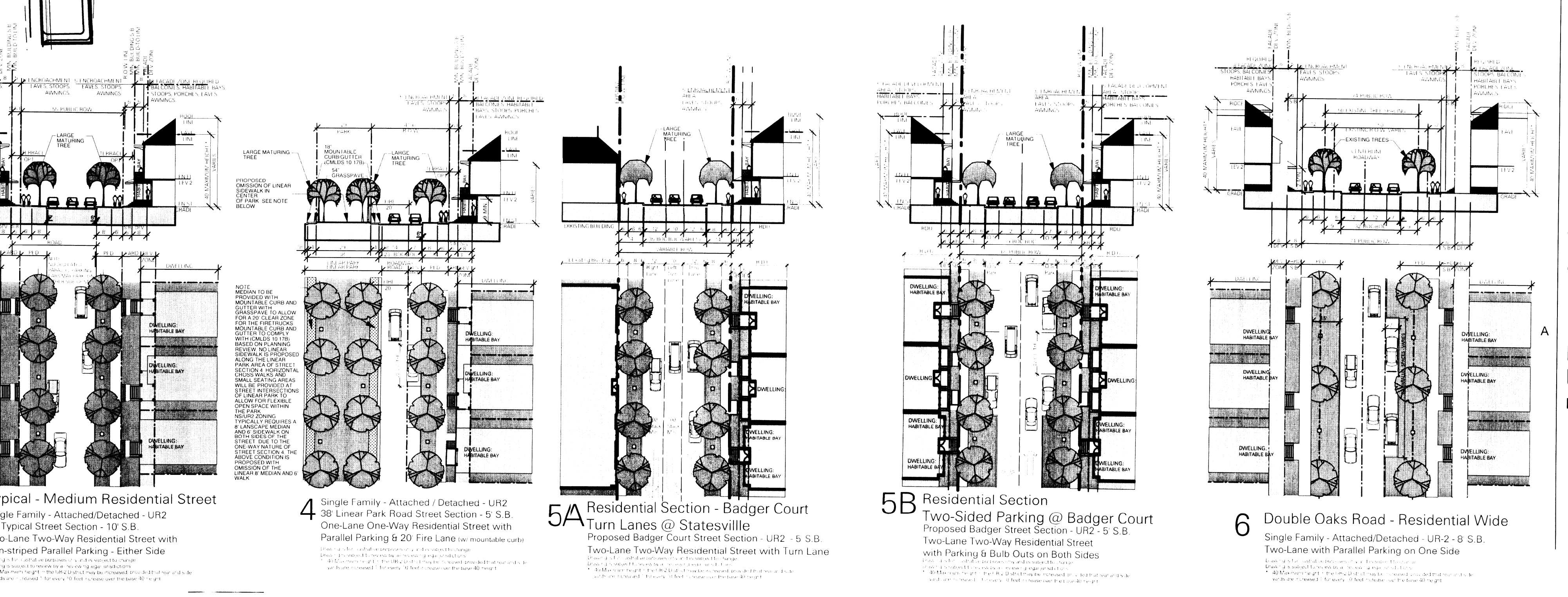
3MU Mixed-Use Street Section Typical Mixed-Use Street Section - NS - Wide - 0 S.B. Two-Lane Two-Way Residential Street with Parallel Parking Both Sides 3.5 Typical - Medium Residential Street Single Family - Attached/Detached - UR2 55 Typical Street Section - 5 S.B. Two-Lane Two-Way Residential Street with Non-striped Parallel Parking - Either Side
