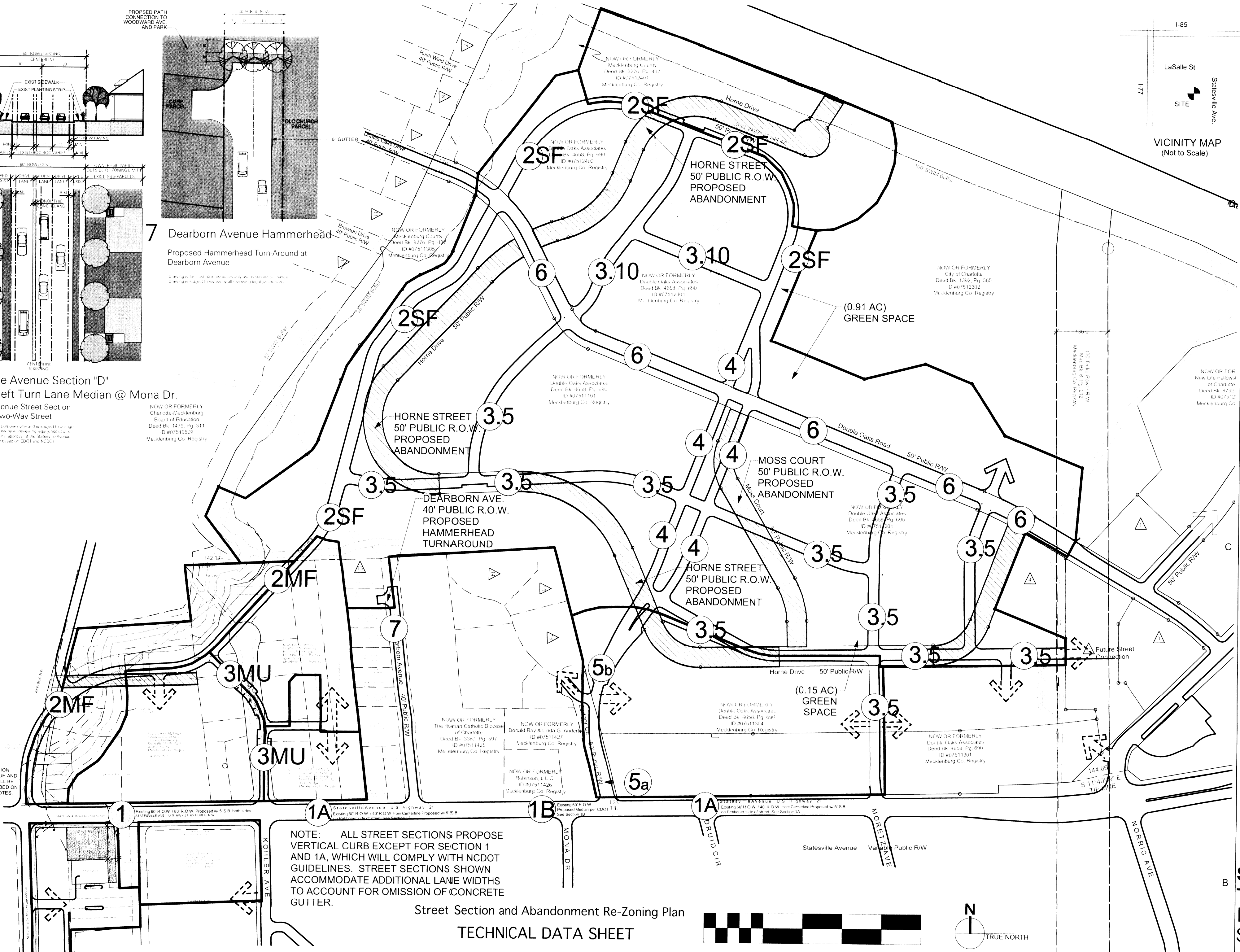
2MF Park Edge - Residential Street Multi Family - Park Edge - NS 55 Anita Stroud & Park Extension Street Section - 5 S.B. Two-Lane Two-Way Residential Street w/ Dedicated On-Street Parking (O Side) 2SF Park Edge - Medium Residential Street Single Family - Attached/Detached - UR2 52 Park Edge Road Street Section - 5 S.B. Two-Lane Two-Way Residential Street with Parallel Parking (non-striped) - Either Side
