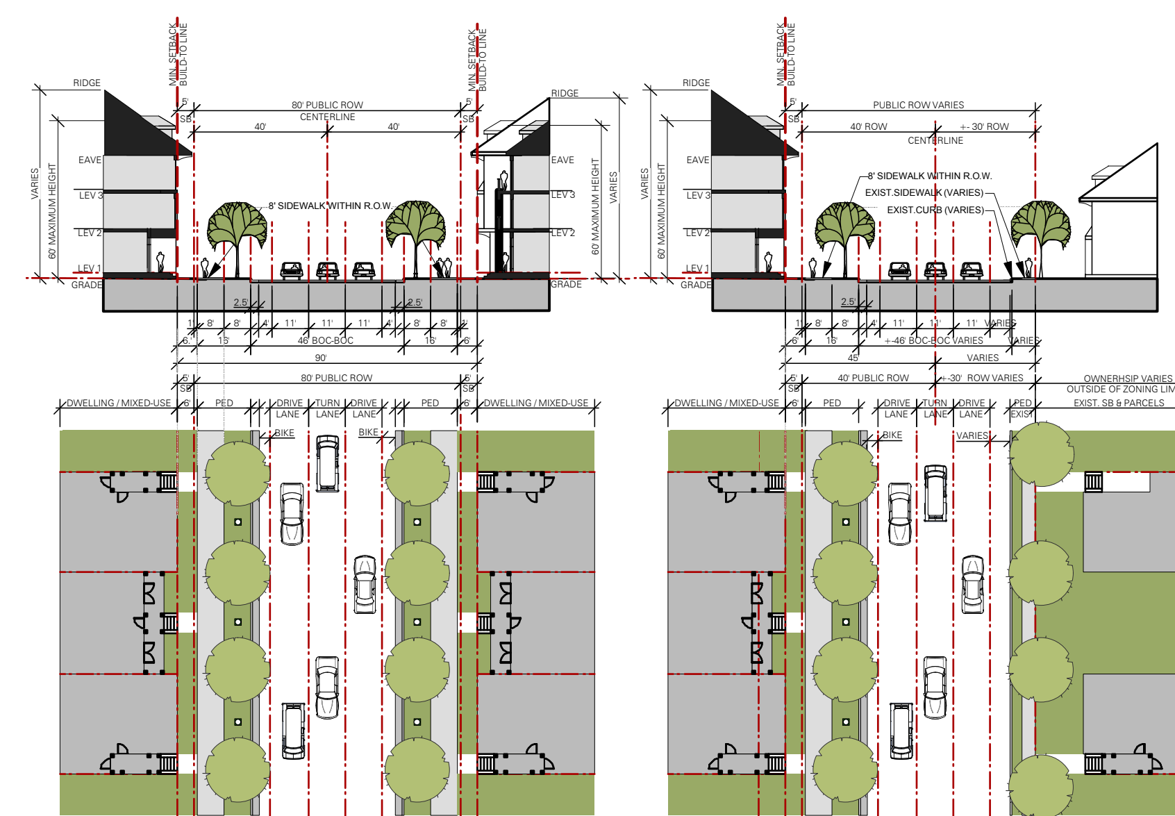
1 Statesville Avenue Petitioner Controls Both Sides Statesville Avenue Street Section - NS Three-Lane Two-Way Street
