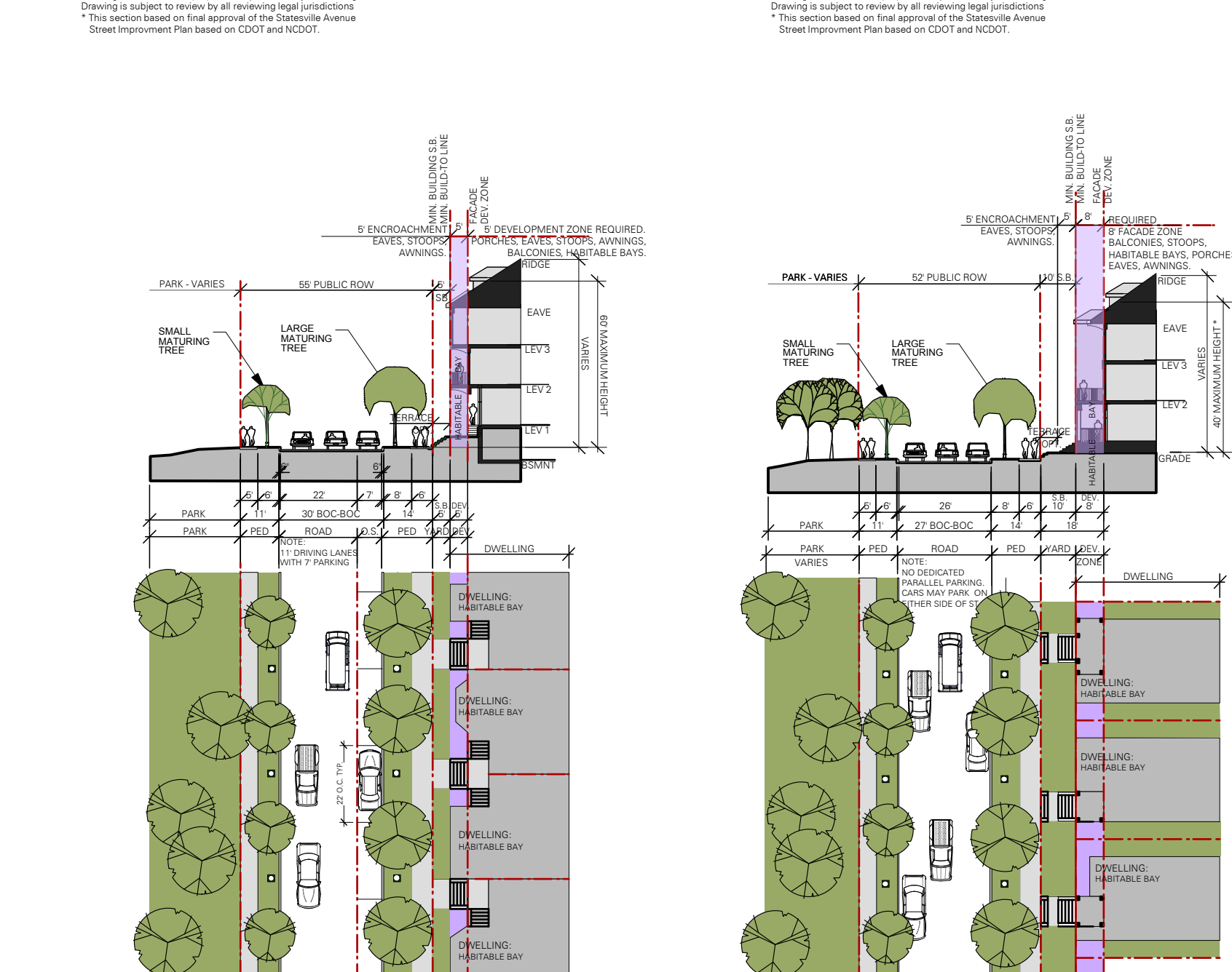
1A Statesville Avenue Petitioner Controls One Side Statesville Avenue Street Section - UR2 Three-Lane Two-Way Street
