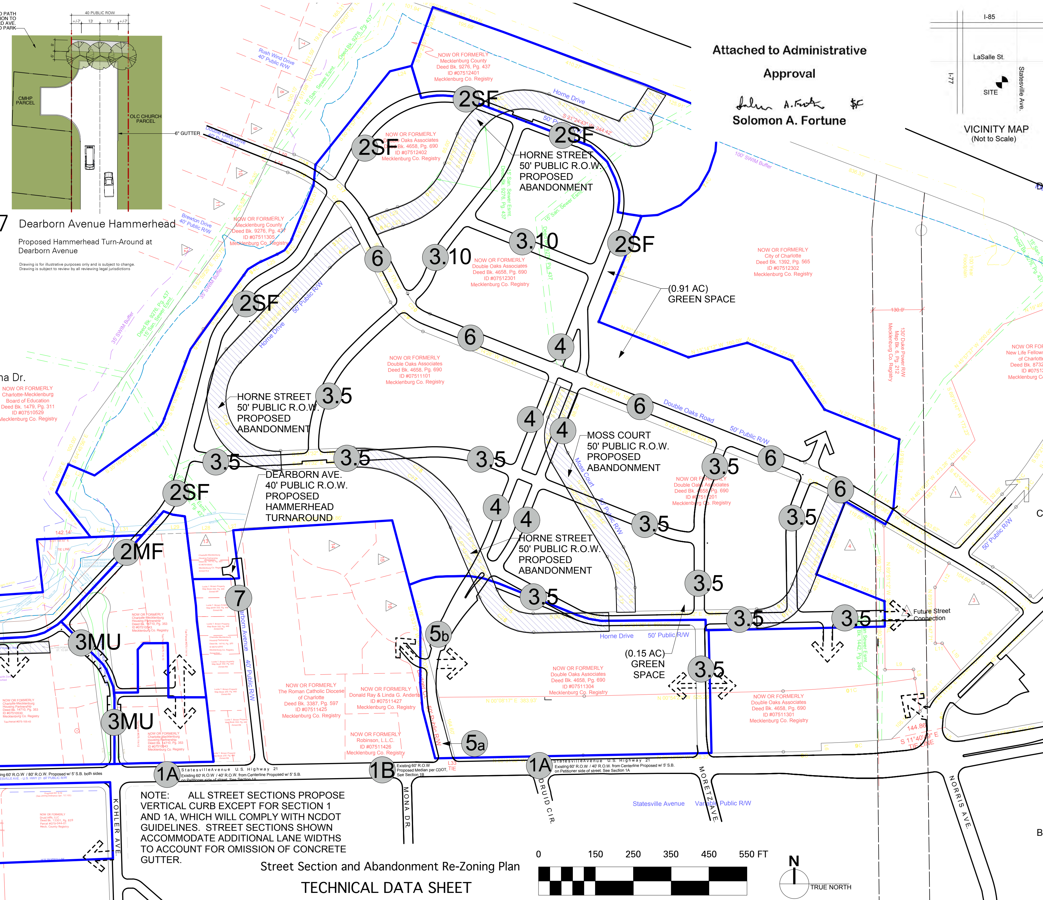
7 Dearborn Avenue Hammerhead Proposed Hammerhead Turn-Around at Dearborn Avenue
