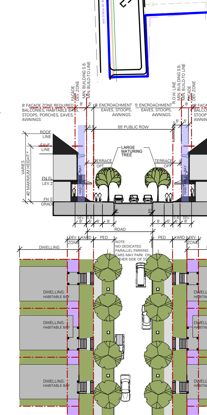
2SF Park Edge - Medium Residential Street Single Family - Attached/Detached - UR2 52 Park Edge Road Street Section - 10' S.B. Two-Lane Two-Way Residential Street with Parallel Parking (non-striped) - Either Side
