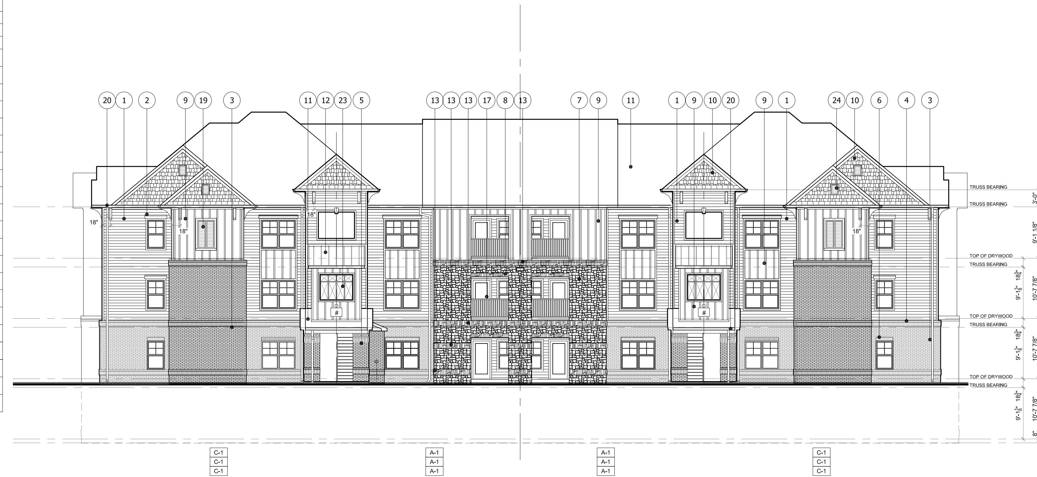
1 TYPE 4 (BLDGs - 3, 4, 5 & 7) - FRONT ELEVATION AS SHOWN 3/27/16 @ 1:00 PM
