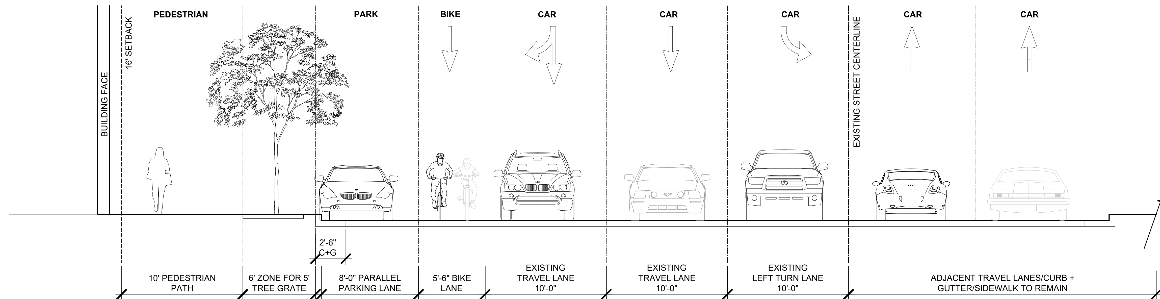
SECTION B - WEST BOULEVARD SCALE: 1/4" = 1'-0"
