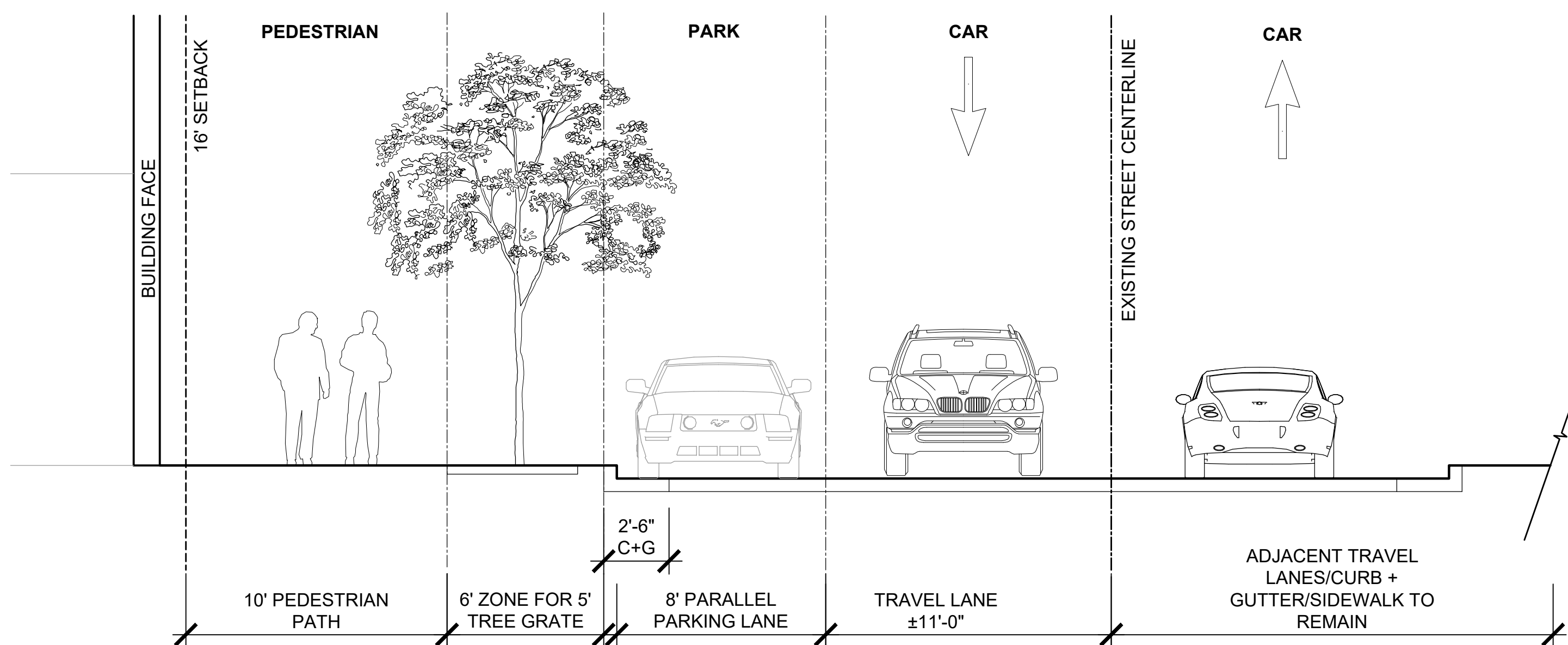
SECTION C - HAWKINS STREET SCALE: 1/4" = 1'-0"
