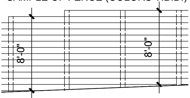
2 PRIVACY FENCE 1/2" = 1'-0"
