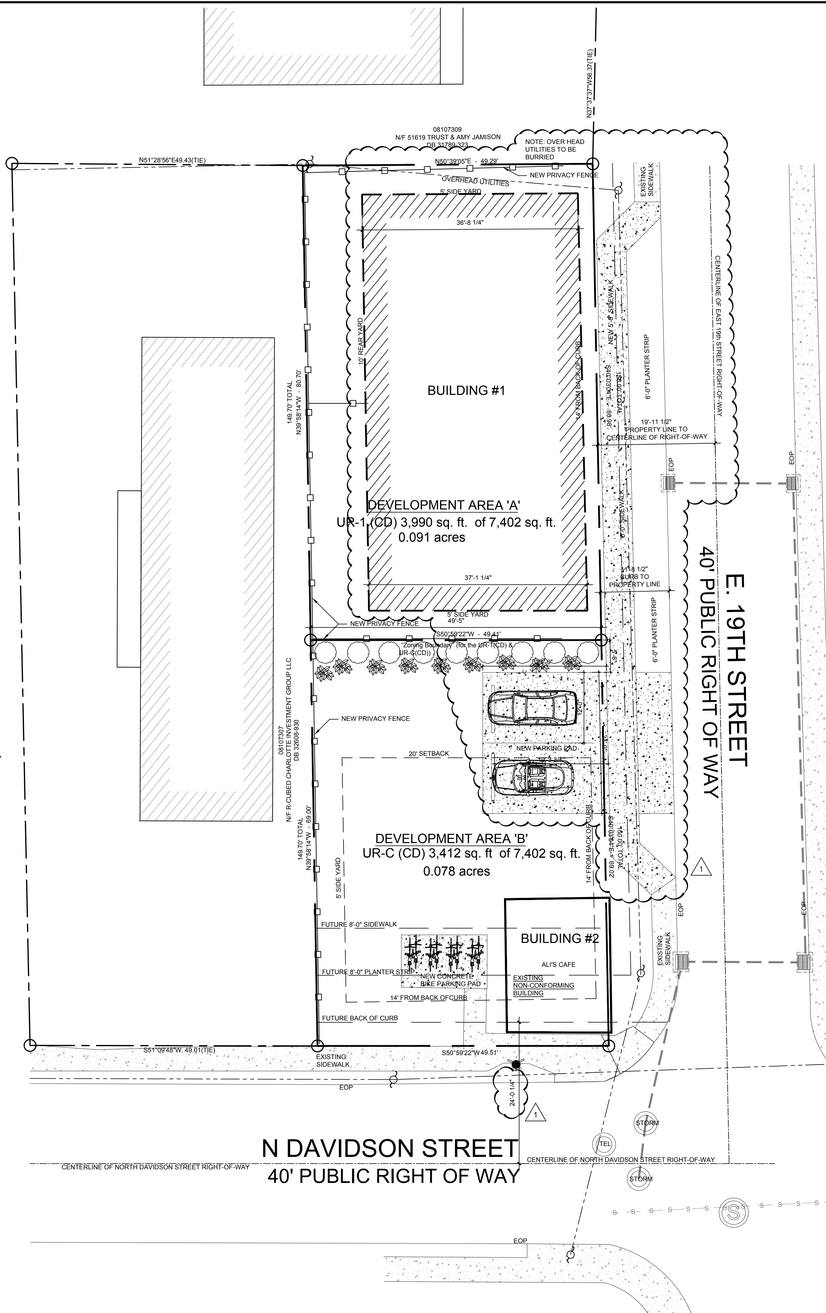
1 PROPOSED SITE PLAN 1" = 10'-0"
