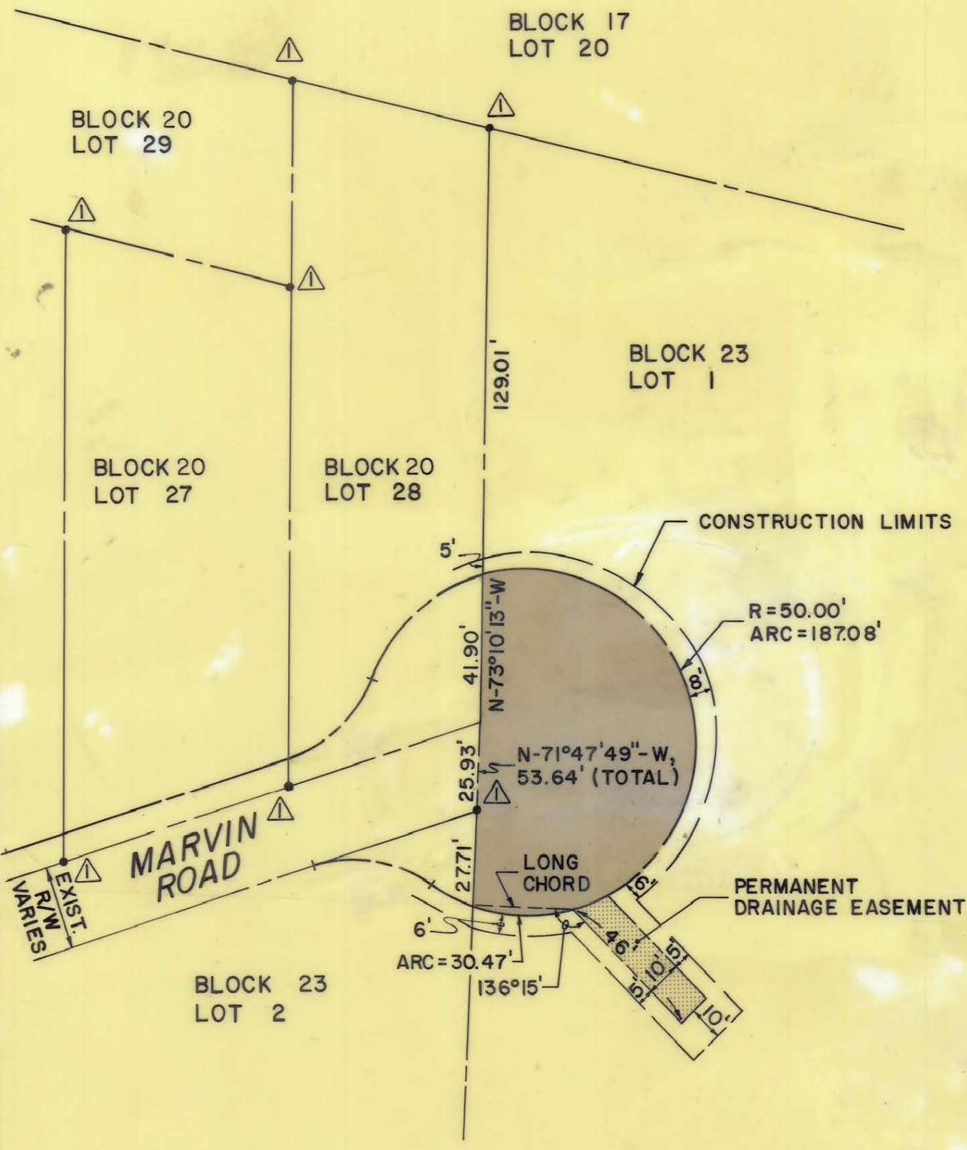
DETAIL 'A'
