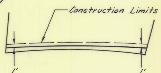
DETAIL 'A'
