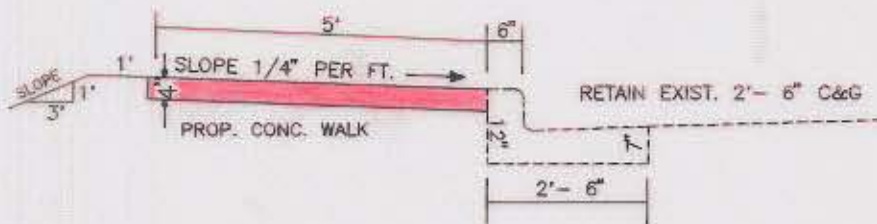
TYPICAL SECTION NTS
