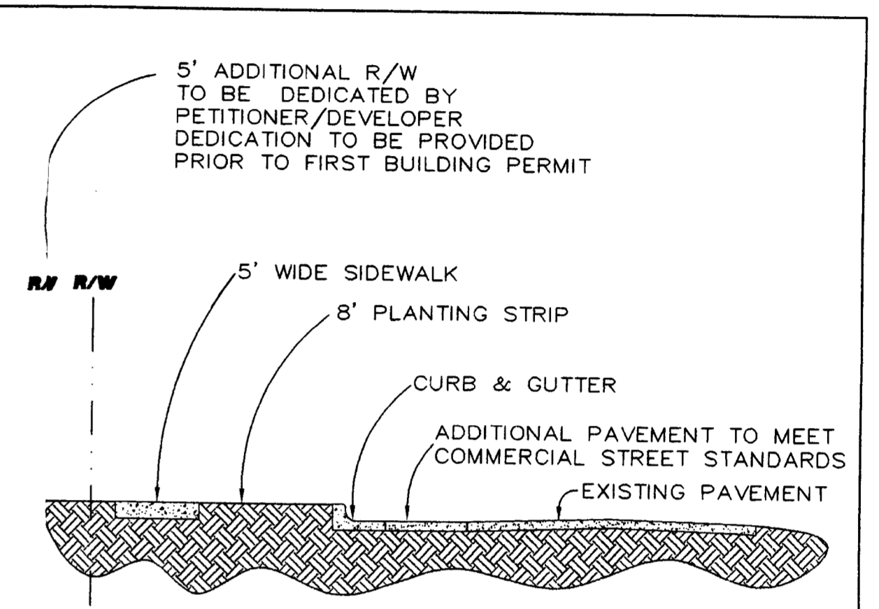
TYPICAL SECTION FOR JOHN ADAMS AND GALLOWAY ROAD I.T.S.
