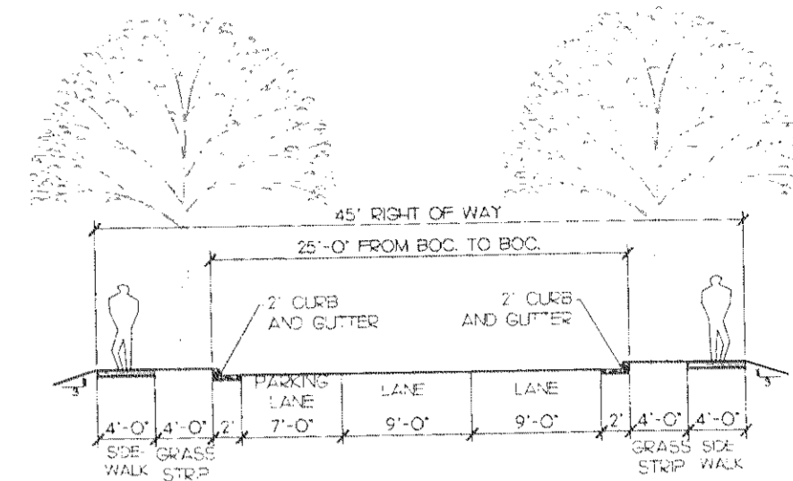
CC PUBLIC RESIDENTIAL ROAD (LOCAL RESIDENTIAL LDS=10.0IG) SECTION SCALE: NTS
