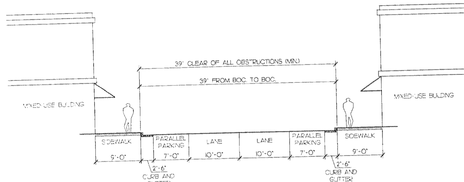
BB PRIVATE MIXED-USE ROAD SECTION SCALE: NTS
