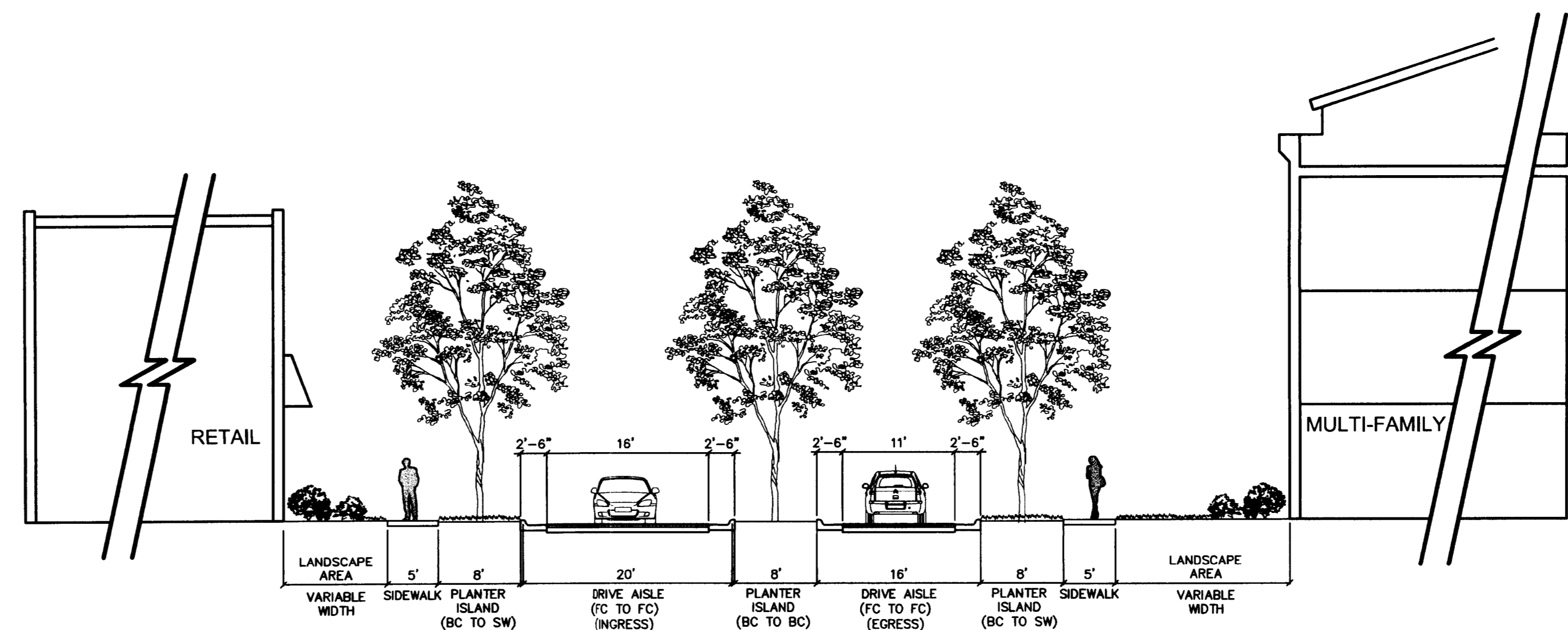
SECTION "C" 1" = 10'
