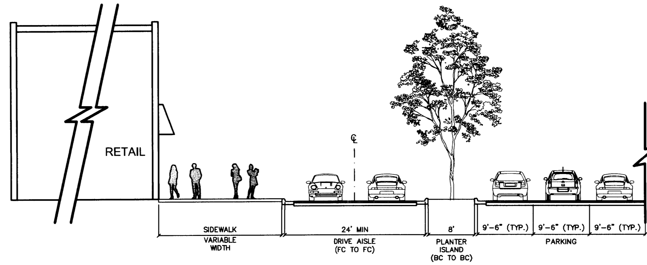
SECTION "A" 1" = 10'
