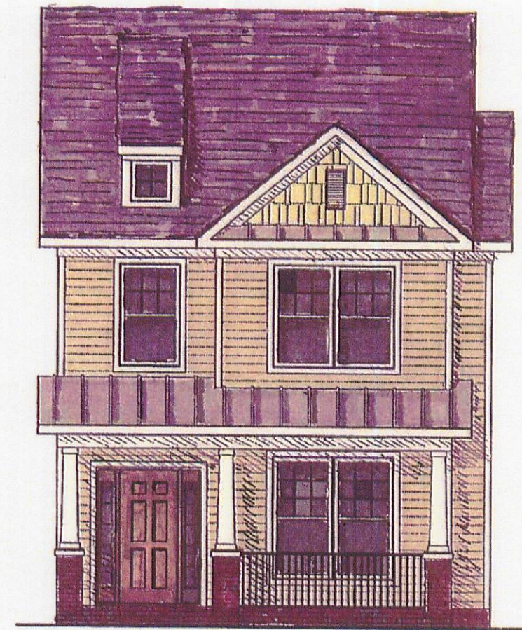
FRONT ELEVATION "Q" SCALE: 1/8"=1'-0" (11"x17" SHEET SIZE) SCALE: 1/4"=1'-0" (24"x36" SHEET SIZE)
