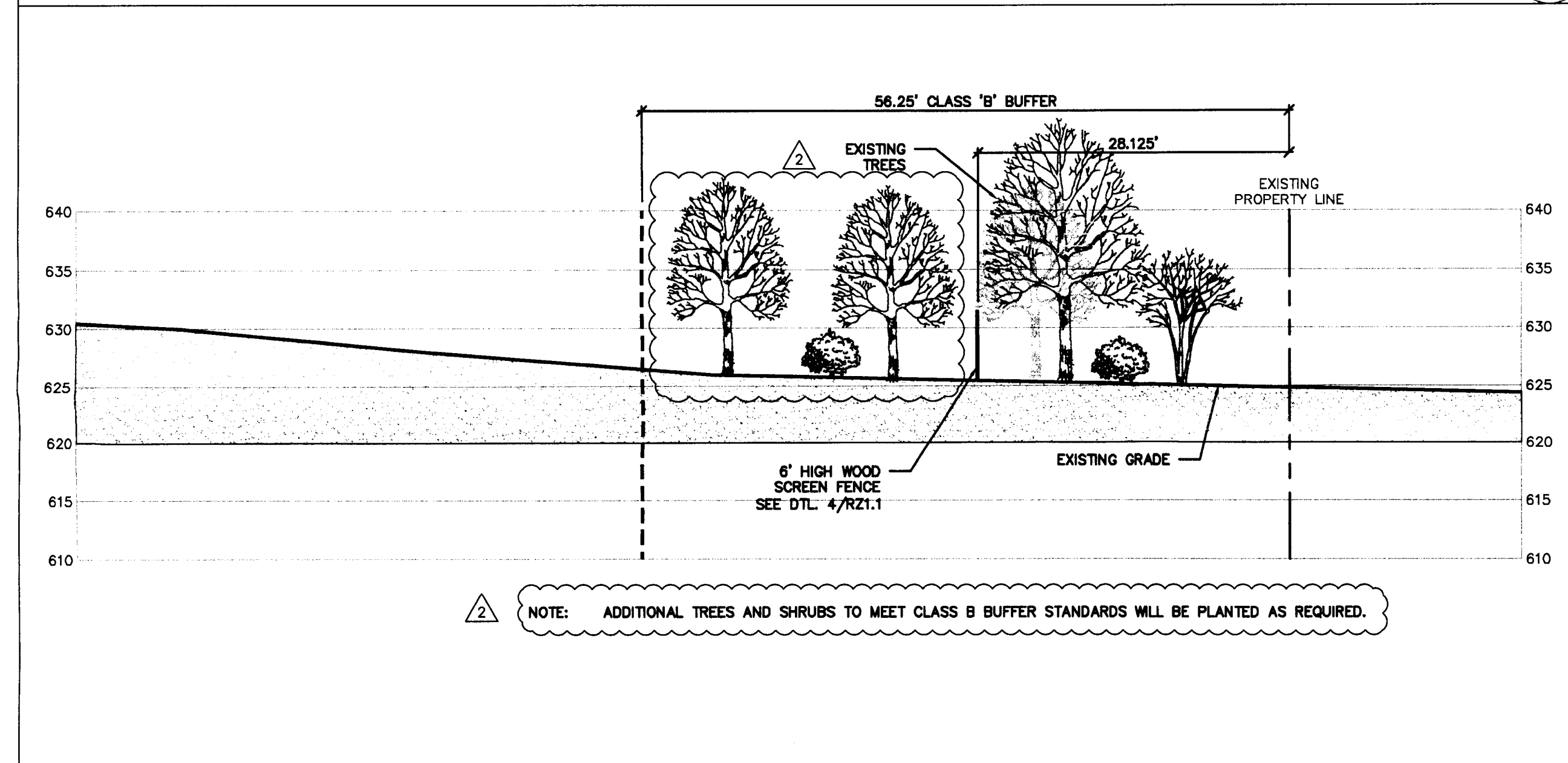
SECTION B-B SCALE 1"=10' 2
