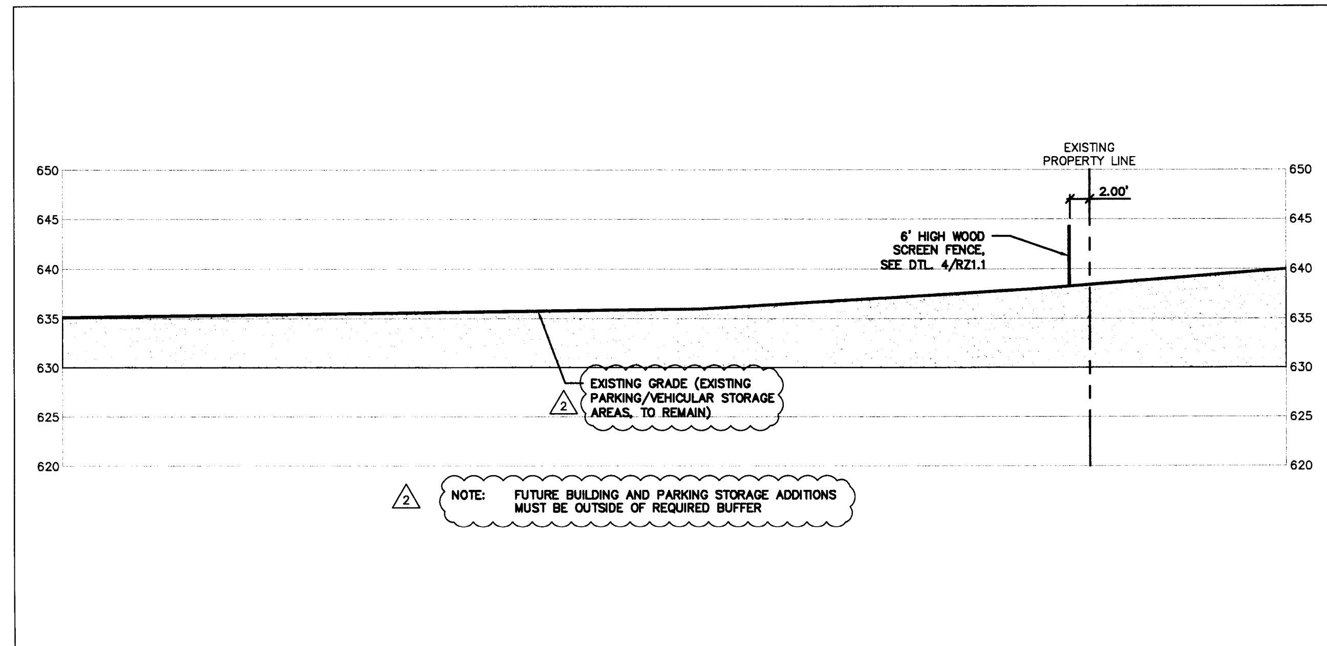
SECTION C-C SCALE 1"=10' 3
