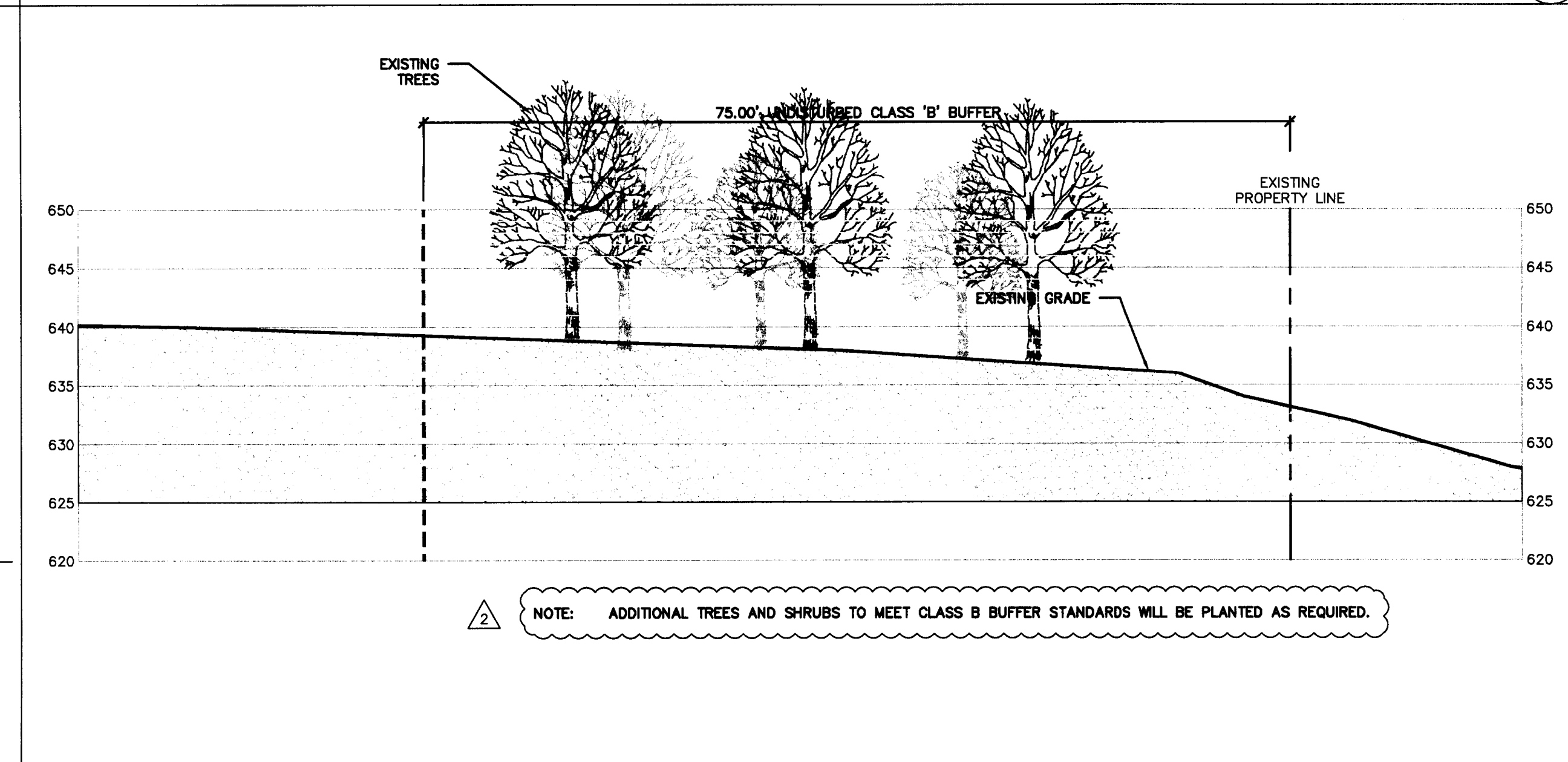
SECTION A-A SCALE 1"=10' 1
