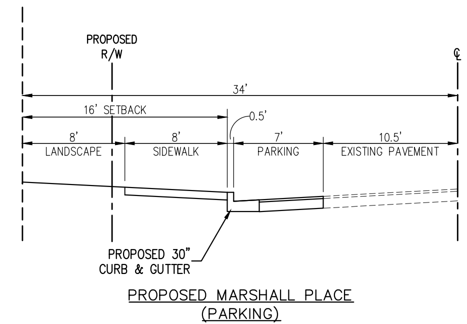
MARSHALL PLACE ROAD SECTION N.T.S.
