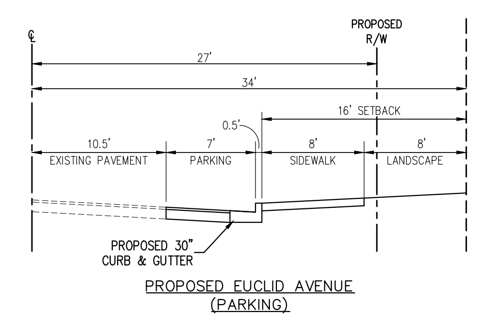
EUCLID AVENUE ROAD SECTION N.T.S.
