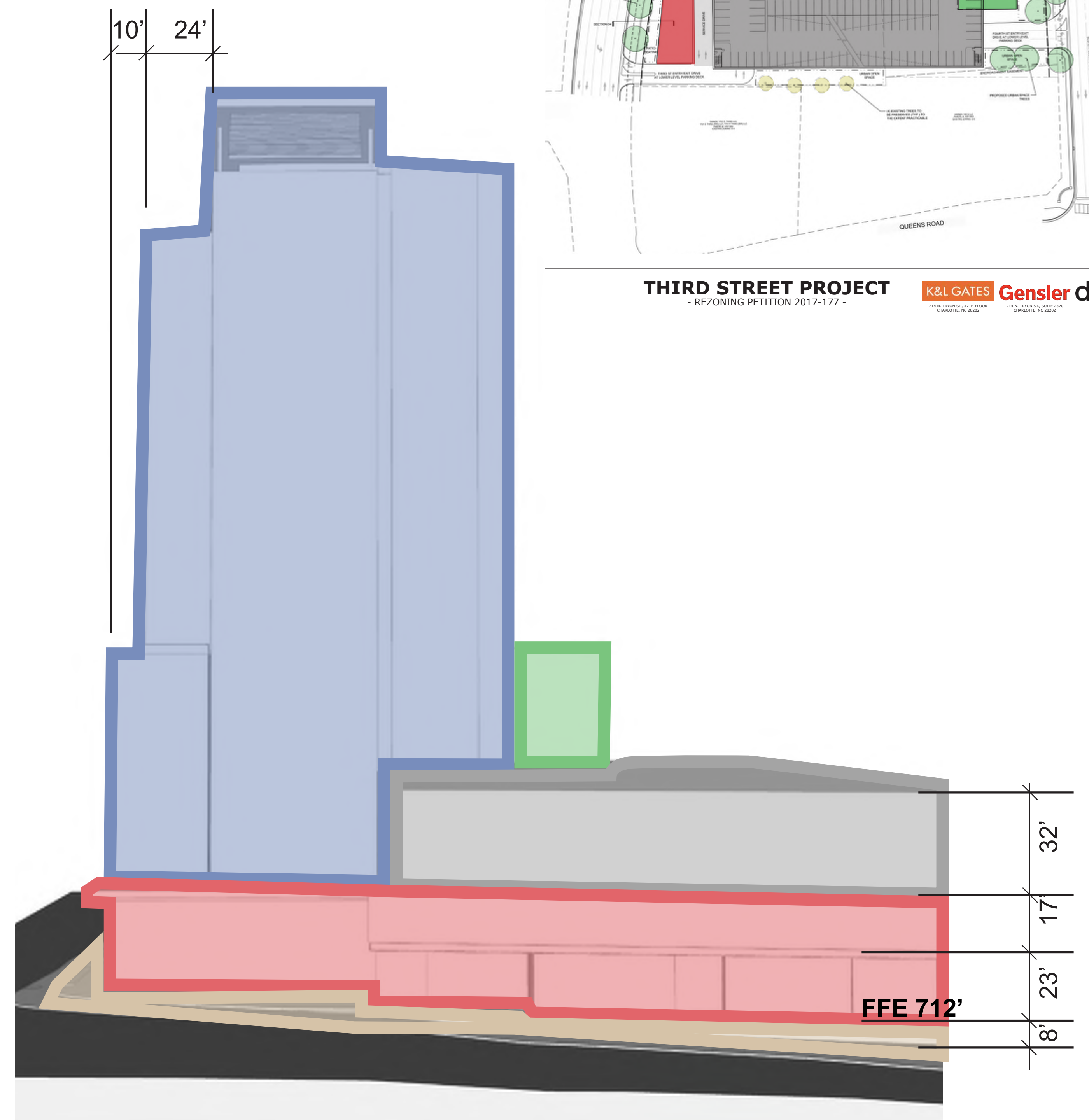
BUILDING MASSING ELEVATION VIEW FROM THIRD STREET
