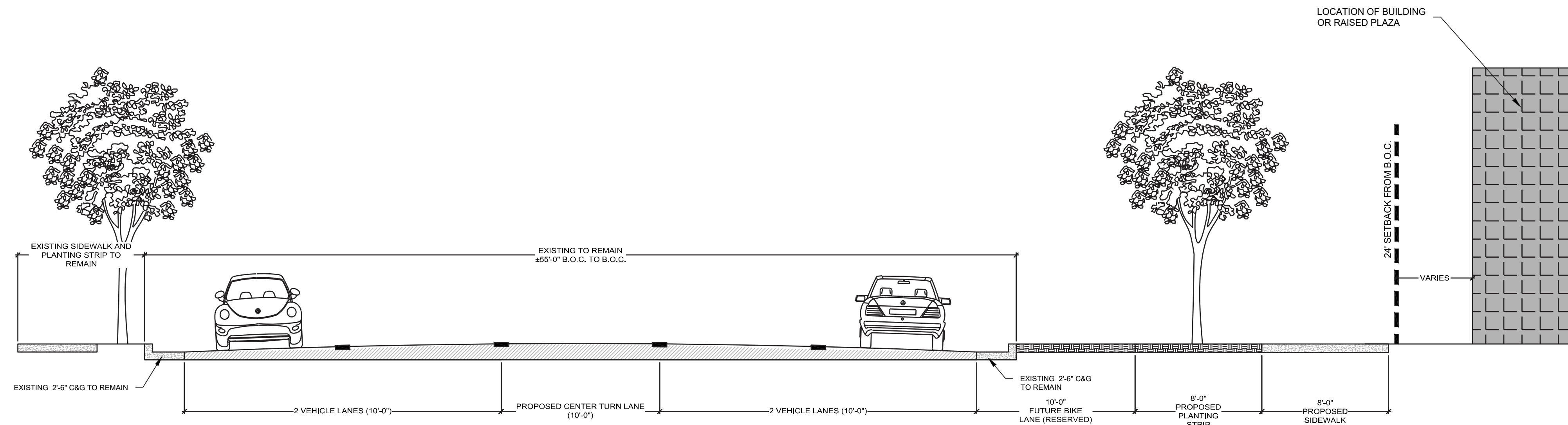
SECTION 05/PROPOSED E. THIRD STREET SECTION NOTE: PROPOSED SECTION SUBJECT TO NCDOT
